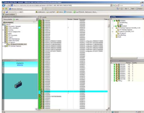
DBWorks WebClient
